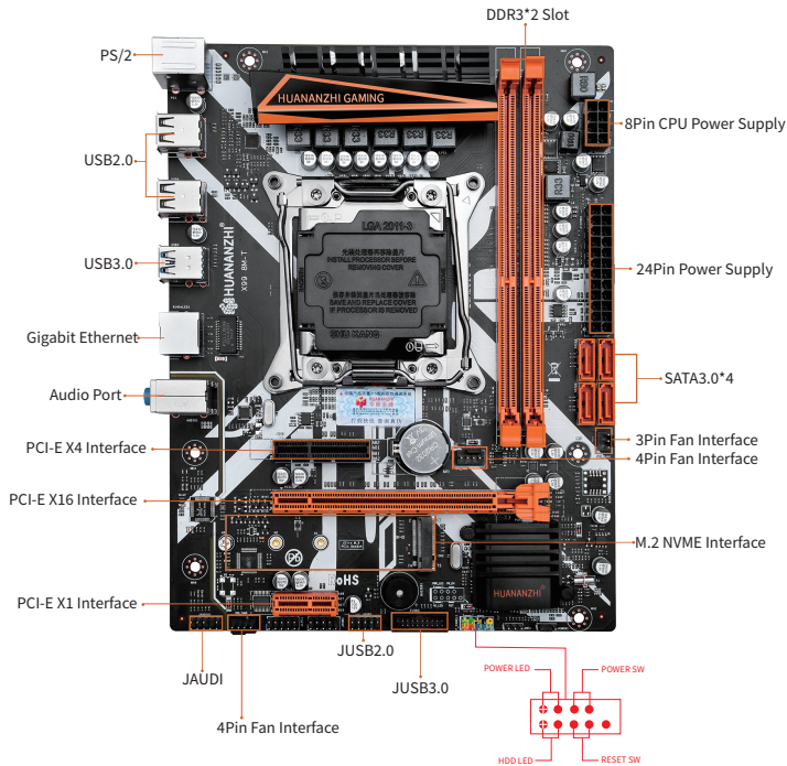
1-1 X99-8M-T Motherboard Illustration
